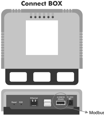
Connect Box Modbus Connector
